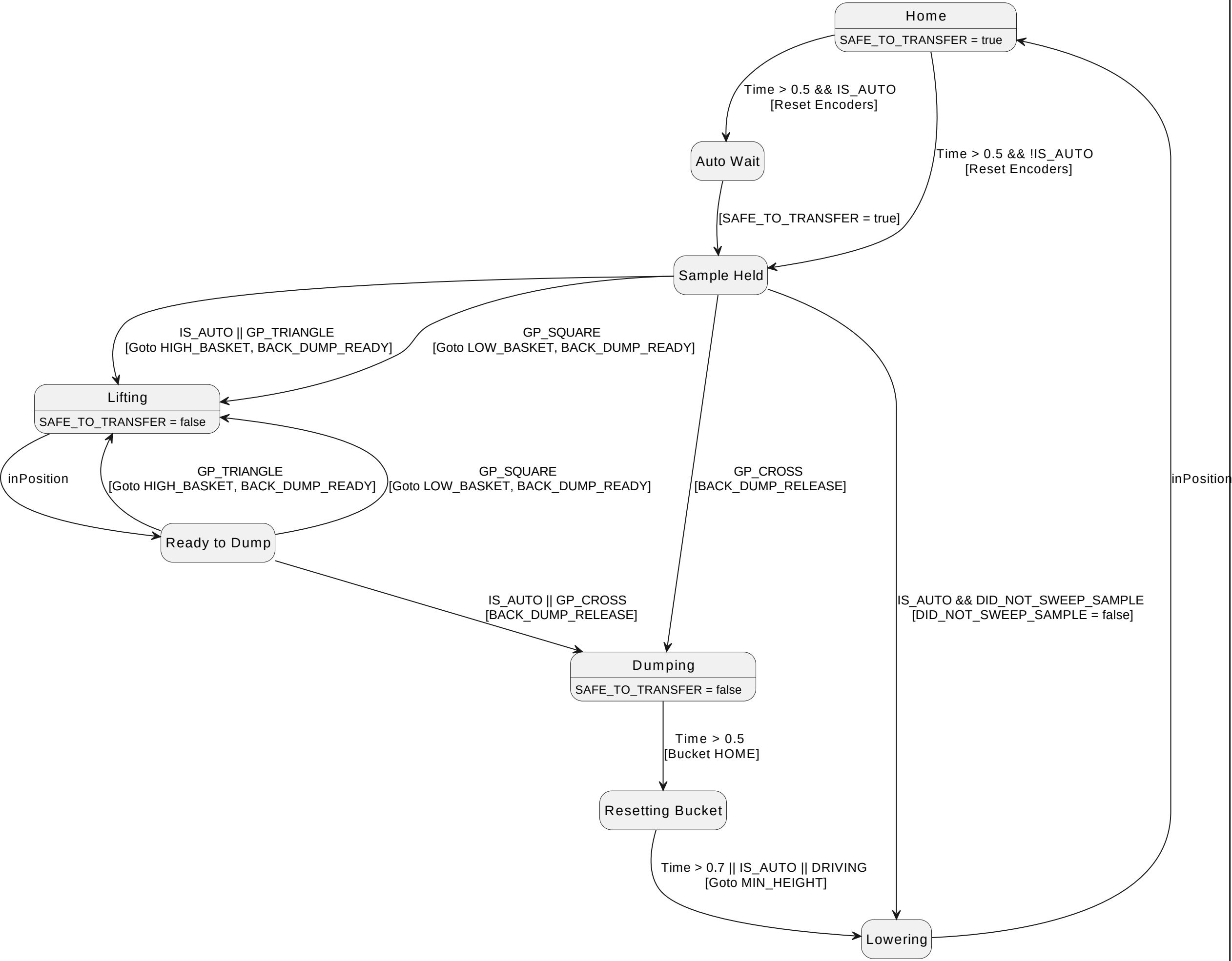
Lift Subsystem State Diagram
